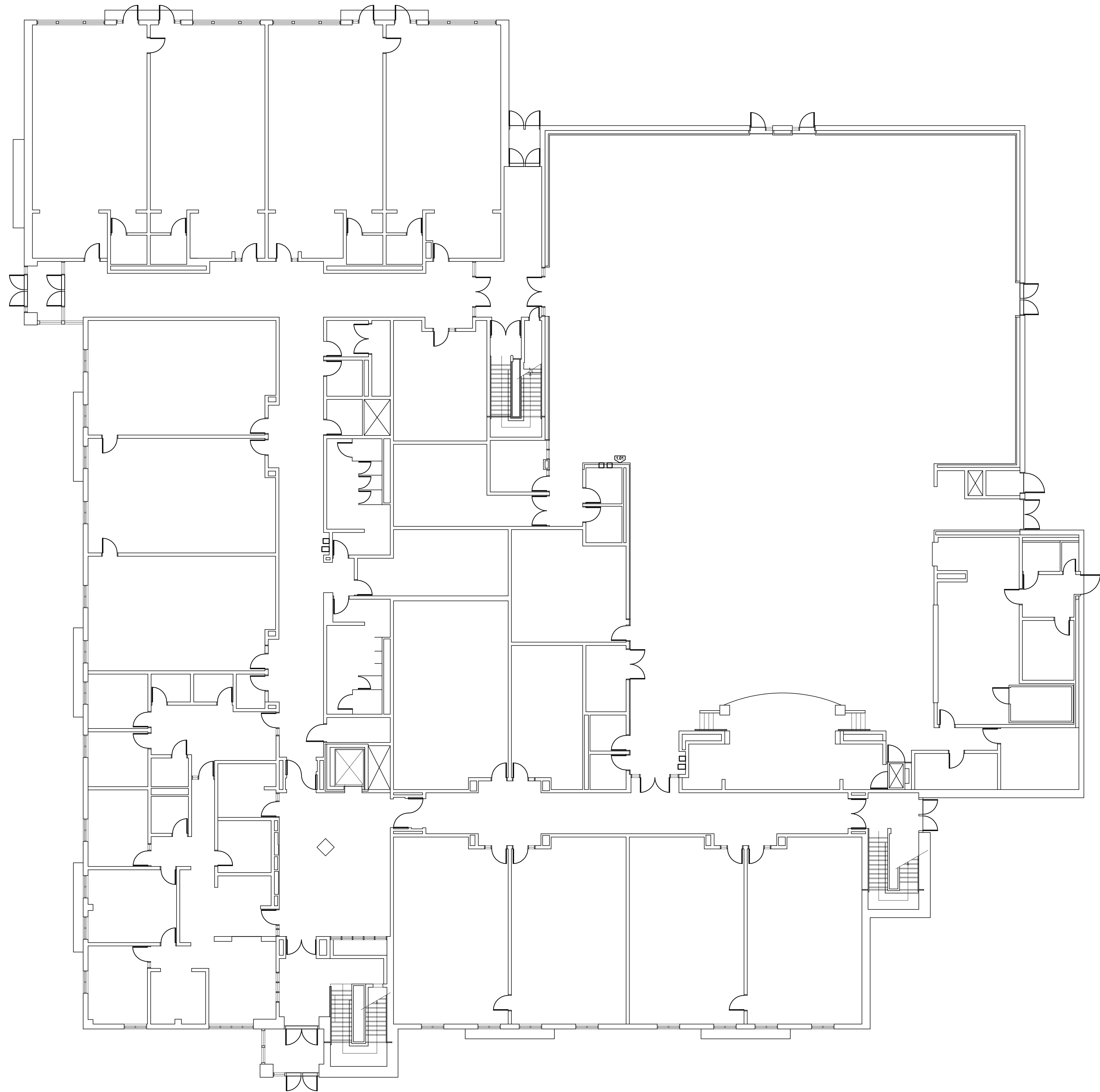
1 FIRST FLOOR SIGNAGE PLAN SCALE: 3/32" = 1'-0"
