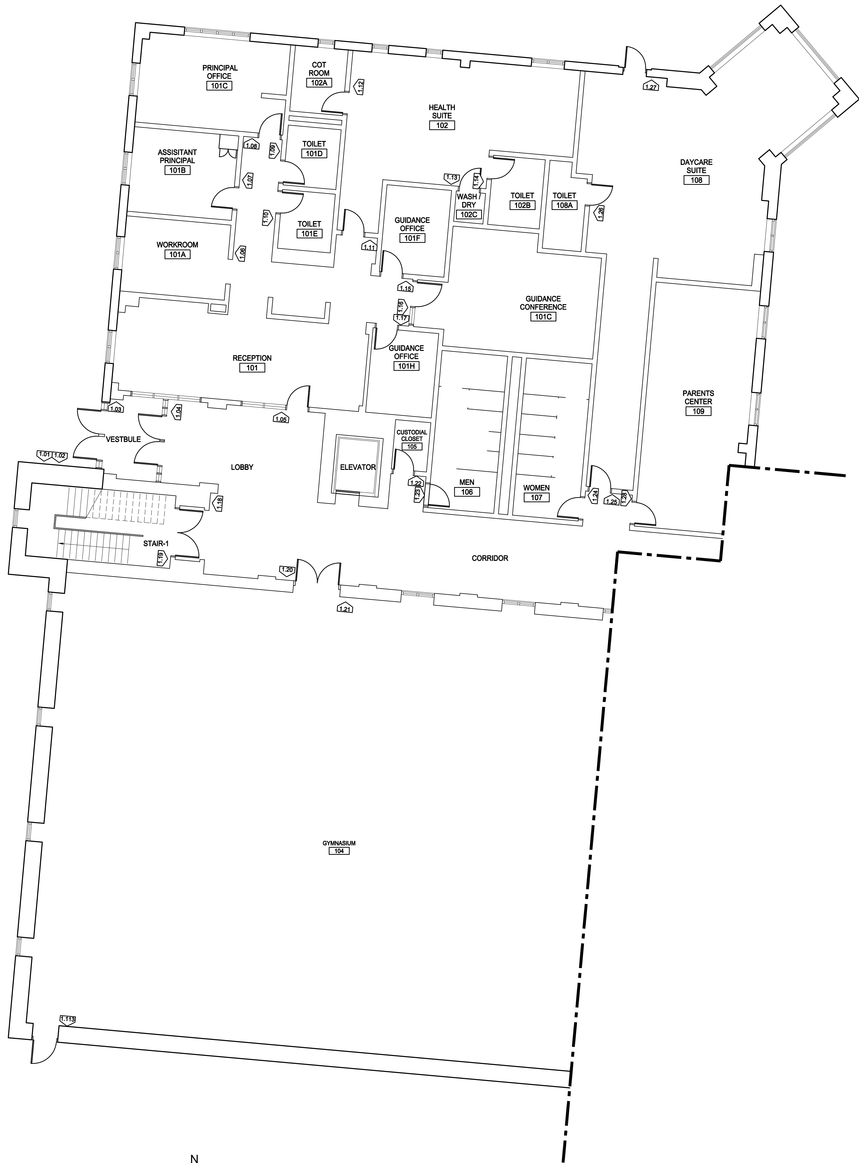
1 FIRST FLOOR SIGNAGE PLAN PART 1 OF 3
